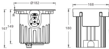
Physical Dimension(MM)
