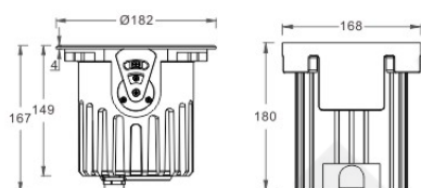
Physical Dimension(MM)
