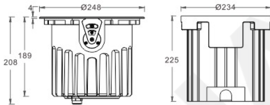
Physical Dimension(MM)
